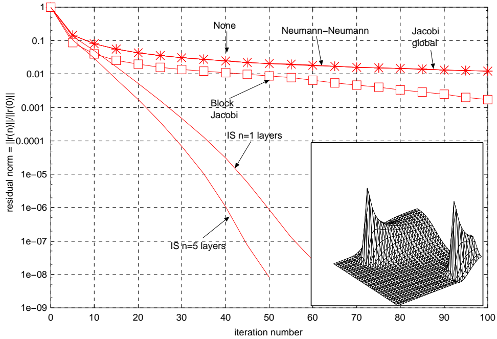
Figure 8. Solution of additive-diffusive problem ( mesh 500 × 500).
