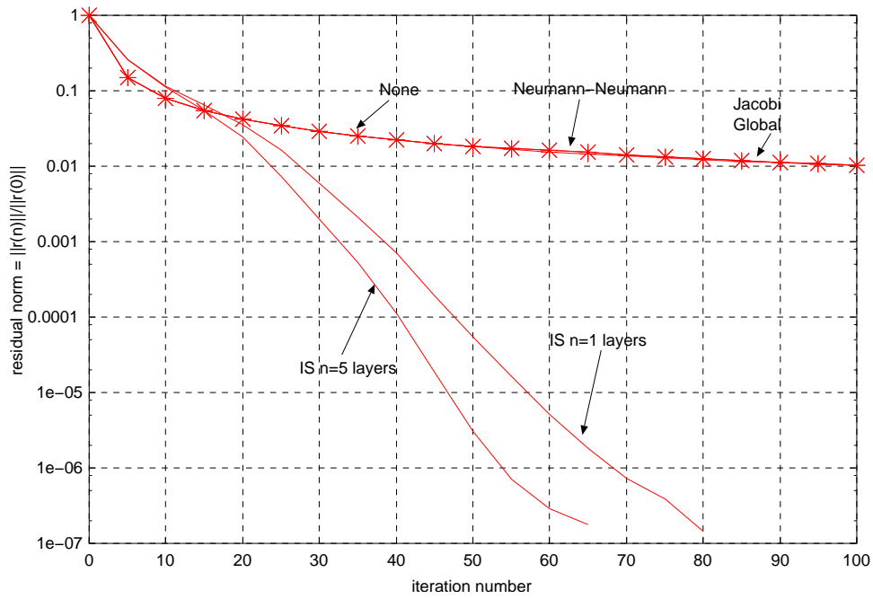
Figure 9. Iteration counts for additive-diffusive problem ( mesh 1000 × 1000).
