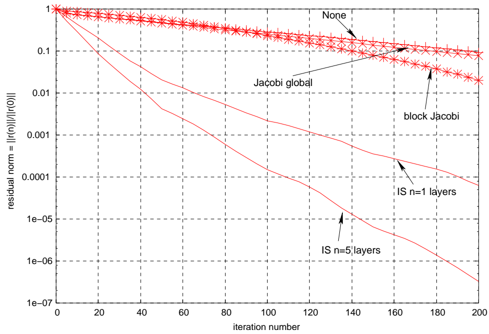
Figure 10. Iteration counts for Saint-Venant system of equations ( mesh 500 × 500).
