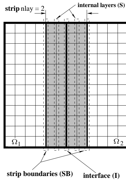
Figure 6. Strip Interface problem.
