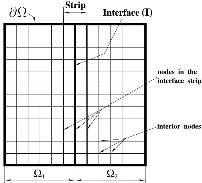
Figure 1. Domain Decomposition.
