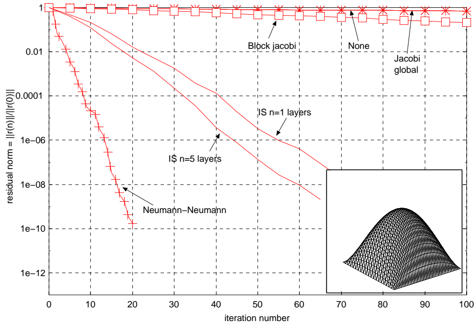
Figure 7. Solution of Poisson's problem ( mesh\ 500 \times 500 ).
