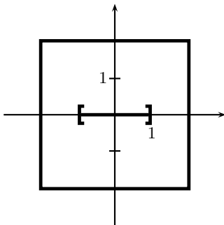
FIGURE 1. X = \{(x, y) \in \mathbb{R}^2 : \bar{d}((x, y), (0, 0)) = 2\} \cup \{(x, 0) : -1 \leq x \leq 1\}
