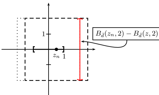
FIGURE 2. B_{\bar{d}}(z_n, 2) - B_{\bar{d}}(z, 2) = \{(2, y) : -2 < y < 2\}
