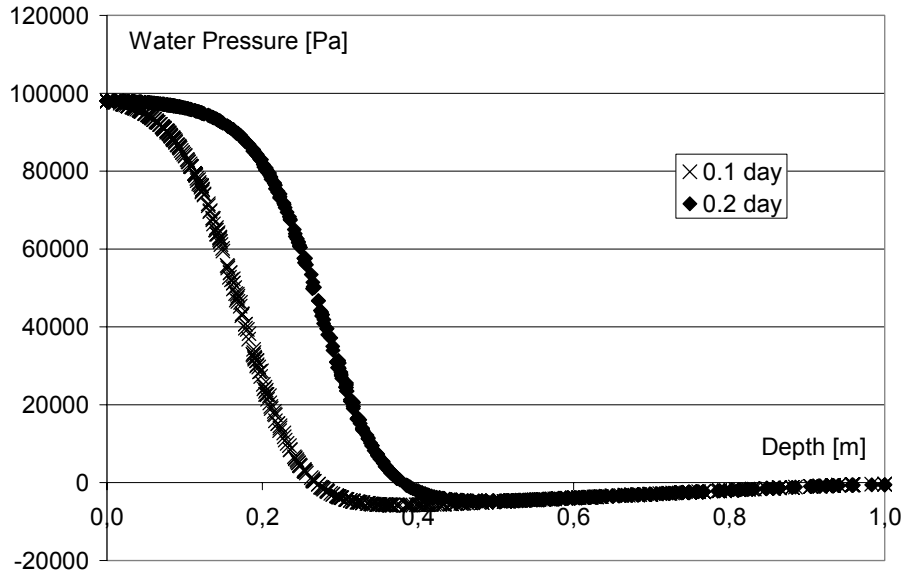
Figure 6: results of case 2 using the 410 subdomains mesh.
