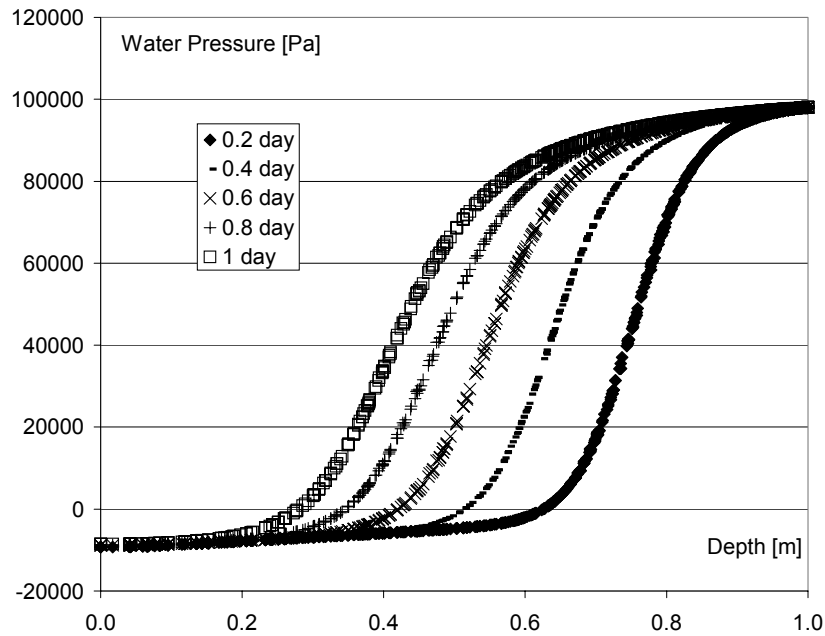
Figure 3: results of case 1.
