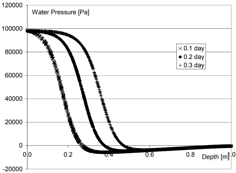
Figure 7: results of case 2 using the 1062 subdomains mesh.
