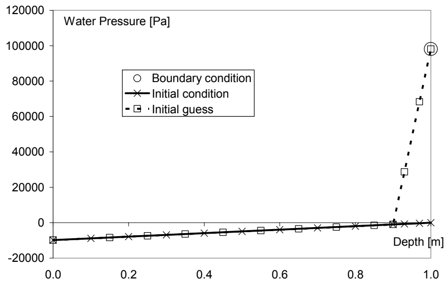
Figure 2: Initial guess and initial condition for case 1.
