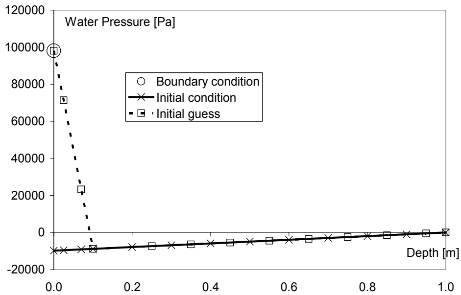
Figure 5: Initial guess and initial condition for case 2.
