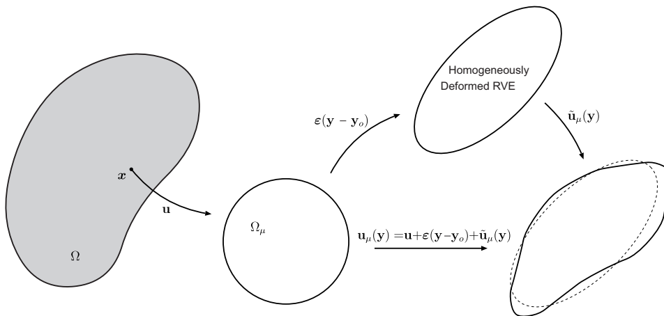
Figure 2: Additive splitting of the microscopic displacement field.
