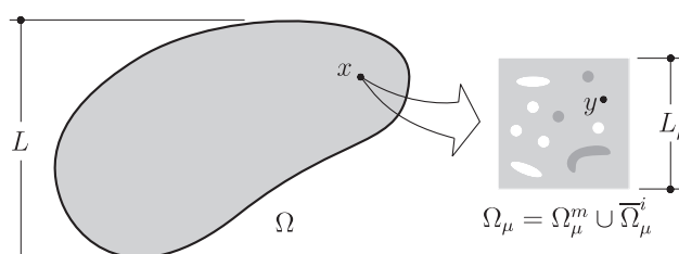
Figure 1: Macroscopic continuum with a locally attached microstructure featuring thermal and mechanical effects.
